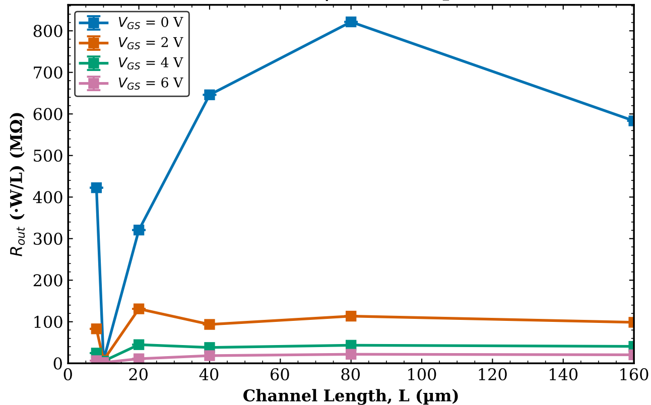
TFT1 Transistor 2 R_{out} vs L | W = 100\text{ }\mu\text{m}
